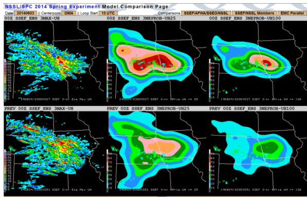
Figure 14. SSEF Day 1 (top row) and Day 2 (bottom row) forecasts of 3-h ensemble maximum UH (left column), ensemble neighborhood probability of UH \geq 25 m/s 2 (middle column), and ensemble neighborhood probability of UH \geq 100 m/s 2 (right column) valid 0000-0300 UTC on 4 June 2014. The severe reports during this 3-h period are plotted as letters in each panel.
