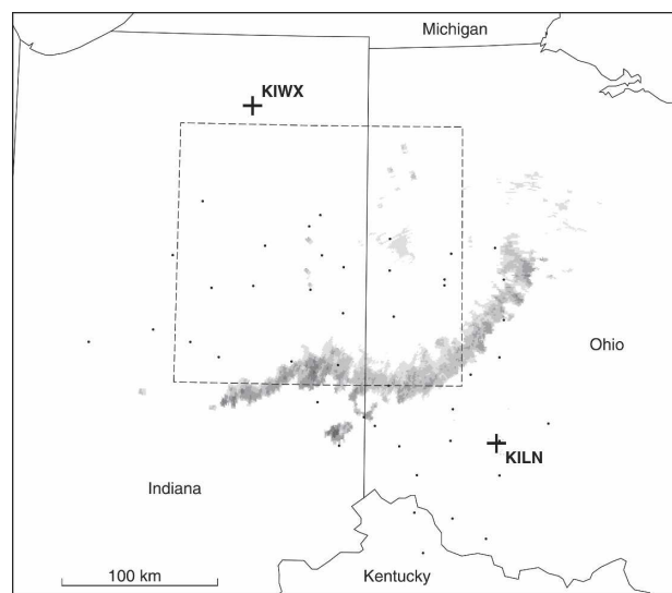
FIG. 10. As in Fig. 4, except at \sim 0045 UTC for the bow echo on 4–5 Jul 2003 over Indiana and Ohio.
