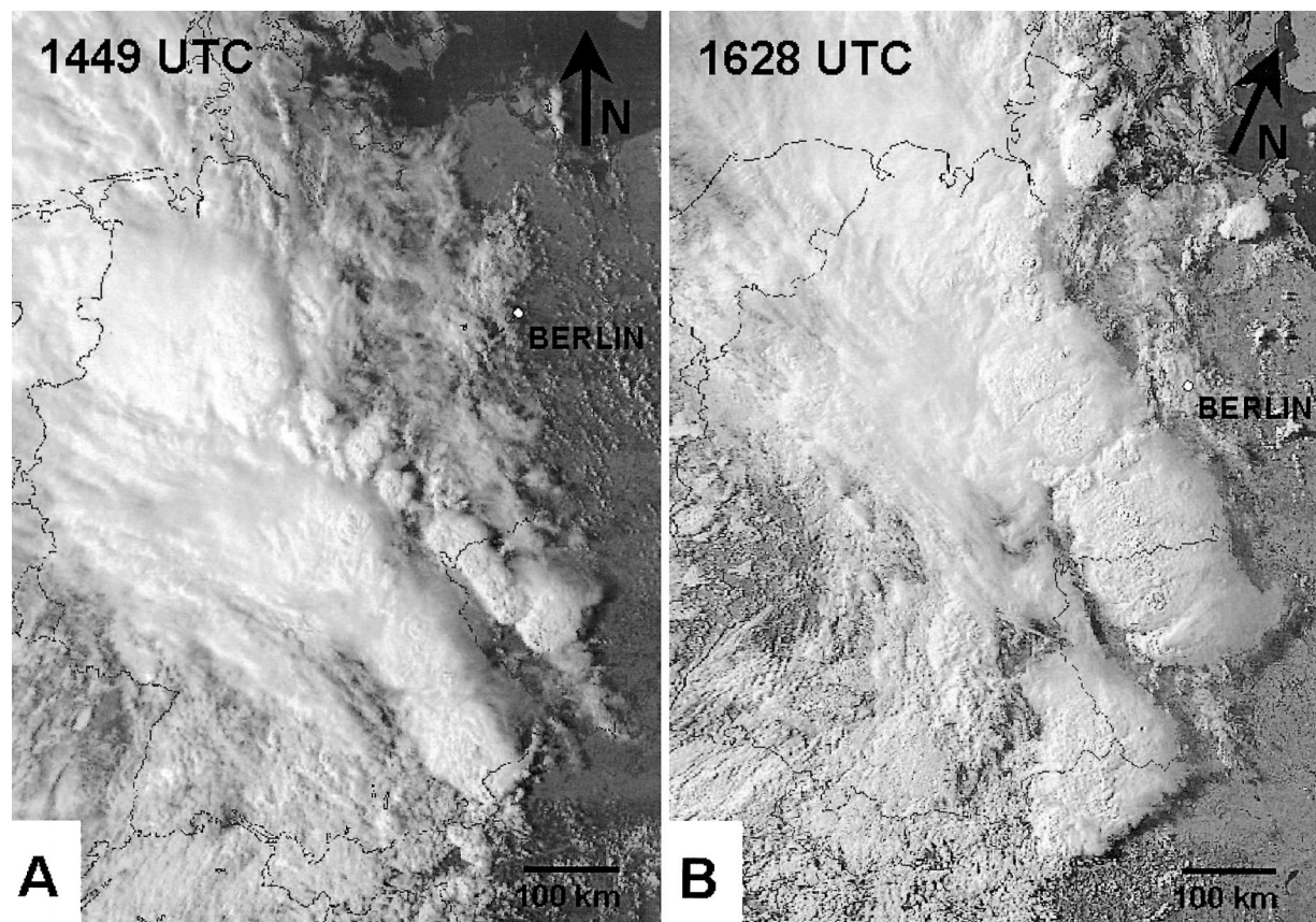
FIG. 3. NOAA satellite visible channel images of Germany at (a) 1449 and (b) 1628 UTC.
