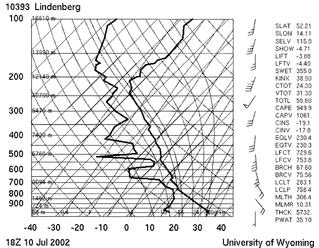
FIG. 5. The 1800 UTC 10 Jul 2002 sounding at Lindenberg in the prestorm environment 40 km southeast of Berlin. Wind barbs are given in kt.
