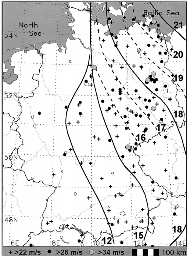
FIG. 8. Measured maximum wind gusts (symbols) and cold front position (lines) over Germany. Wind gusts above 22 \text{ m s}^{-1} are depicted by crosses, above 26 \text{ m s}^{-1} by dots, and above 34 \text{ m s}^{-1} by gray circles. The UTC time of cold front position is shown at the end of each line. Solid lines are plotted every 3 h, with dashed lines of hourly intervals.
