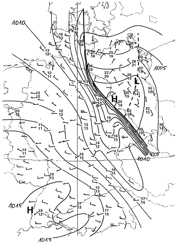
FIG. 4. Subjective analysis of surface pressure field at 1700 UTC based on observations by the German Weather Service. Temperatures and dewpoints in °C and wind barbs in kt.
