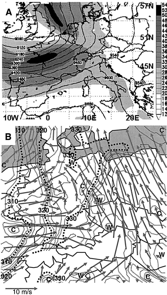
FIG. 1. Operational BOLAM forecast for 1500 UTC 10 Jul 2002. (a) The 300-hPa geopotential (gpm) and wind speed ( \text{m s}^{-1} ). Geopotential heights are shown by black lines; wind speed is indicated by gray shading. (b) The 850-hPa \theta_e field (K) and wind vectors scaled by the 10 \text{ m s}^{-1} vector at the bottom of the figure.
