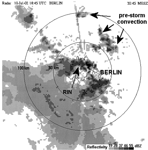
FIG. 7. Radar reflectivity in the Berlin region at 1845 UTC. Arrows point at the rear inflow notch south of the bow echo over Berlin and the developing prestorm convection.
