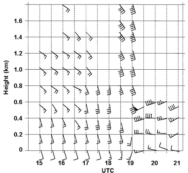
FIG. 6. Wind profiler and sodar data from the German Weather Service at Lindenberg. Wind barbs are given in kt.
