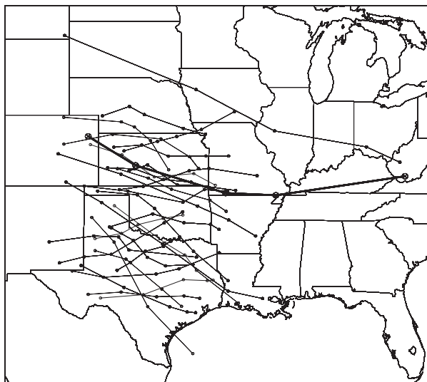
FIG. 3. Paths of the 28 MCSs (thin lines) from C2010 used in the comparison to the 8 May 2009 MCS (thick line). The points along the lines denote the locations of the first storms, genesis, mature, decay, and dissipation stages of the MCSs, respectively (see text for details).
