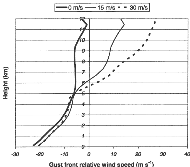
FIG. 18. The gust-front-relative ambient wind profiles for the 3D simulations at 3.5 h. To create the profiles, the u wind component is averaged in an x = 20 km by y = 80 km box centered 20 km ahead of the center portion of the gust front.
