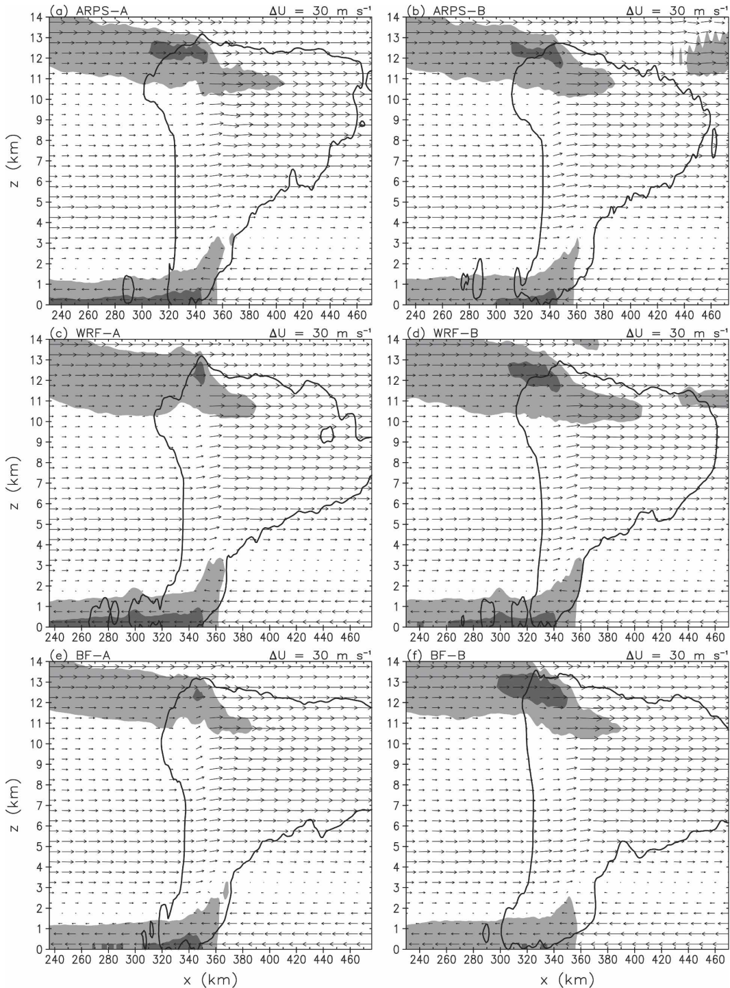
FIG. 4. Same as in Fig. 2, but for \Delta U = 30 \text{ m s}^{-1} .
